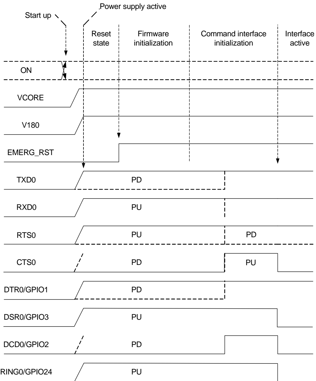
Figure 6: ASC0 startup behavior
