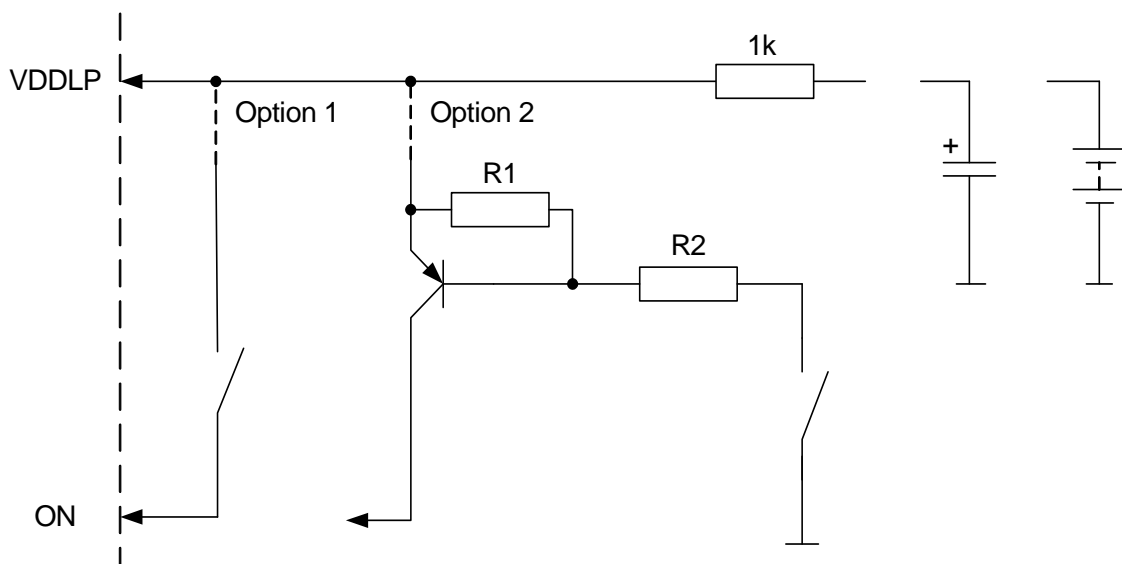
Figure 28: ON circuit sample
