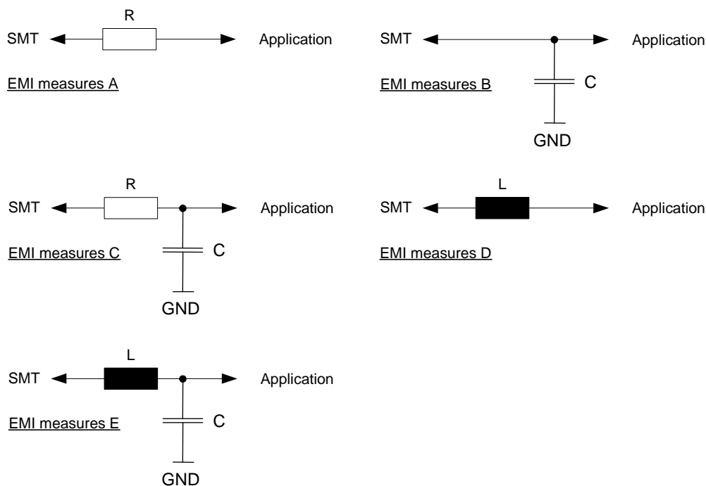
Figure 37: EMI circuits
