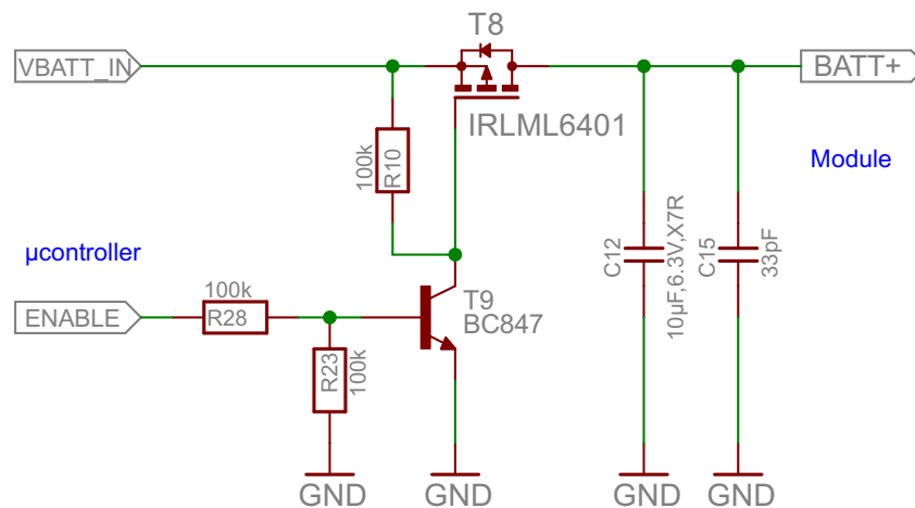
Figure 32: Restart circuit using BATT+ line
