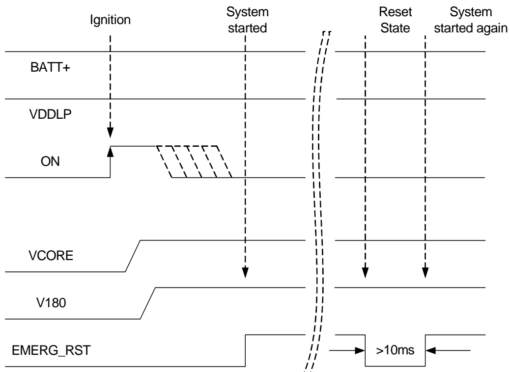
Figure 30: Emergency restart timing
