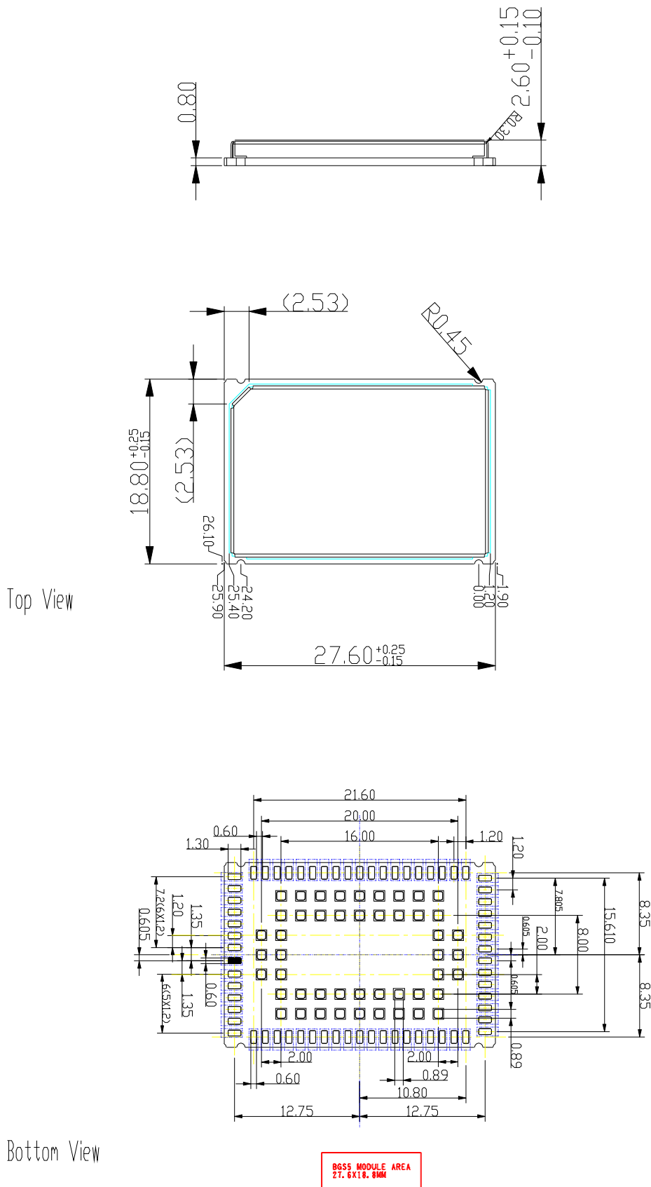
Figure 39: Dimensions of BGS5 (all dimensions in mm)
