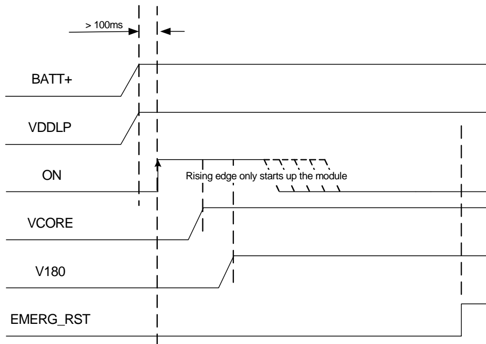
Figure 29: ON timing
