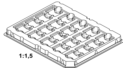
Figure 50: Small quantity tray
