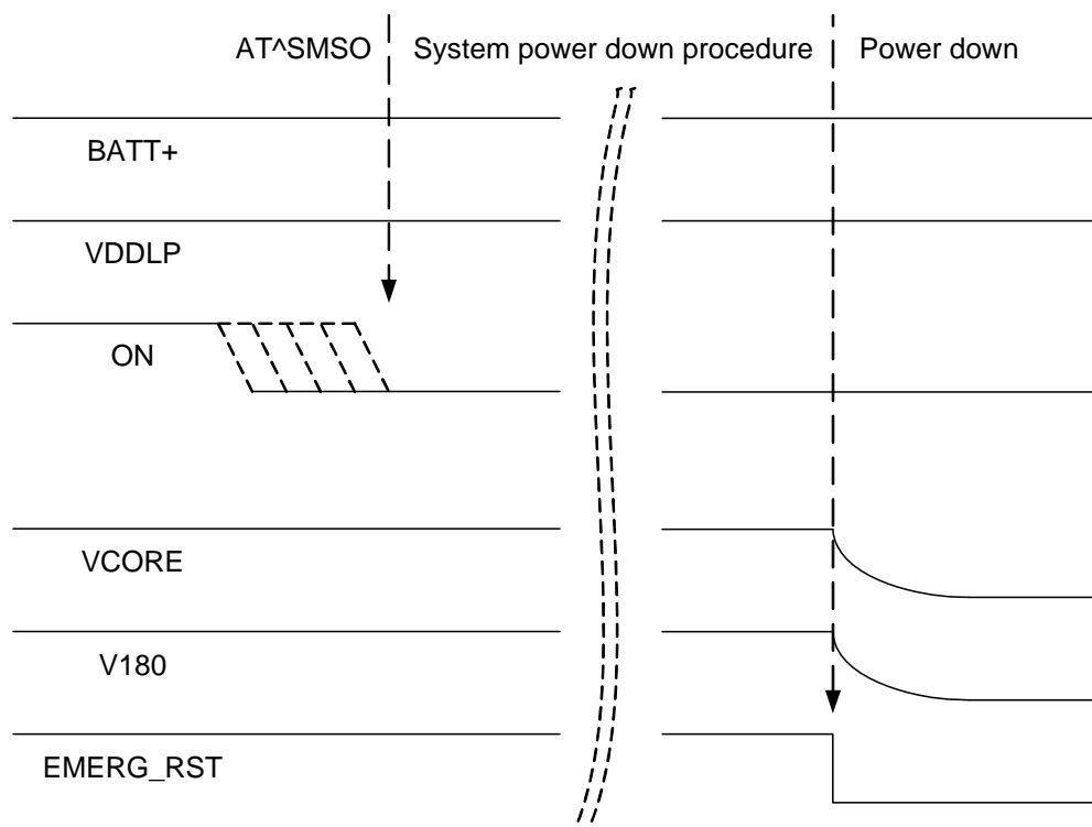
Figure 31: Switch off behavior
