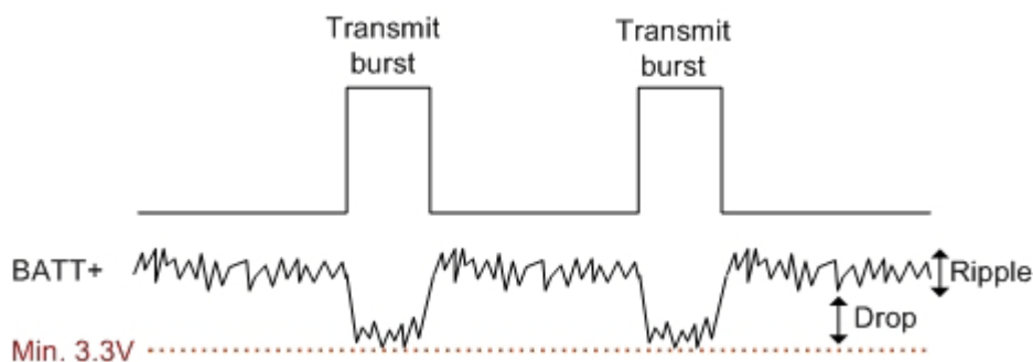
Figure 34: Power supply limits during transmit burst
