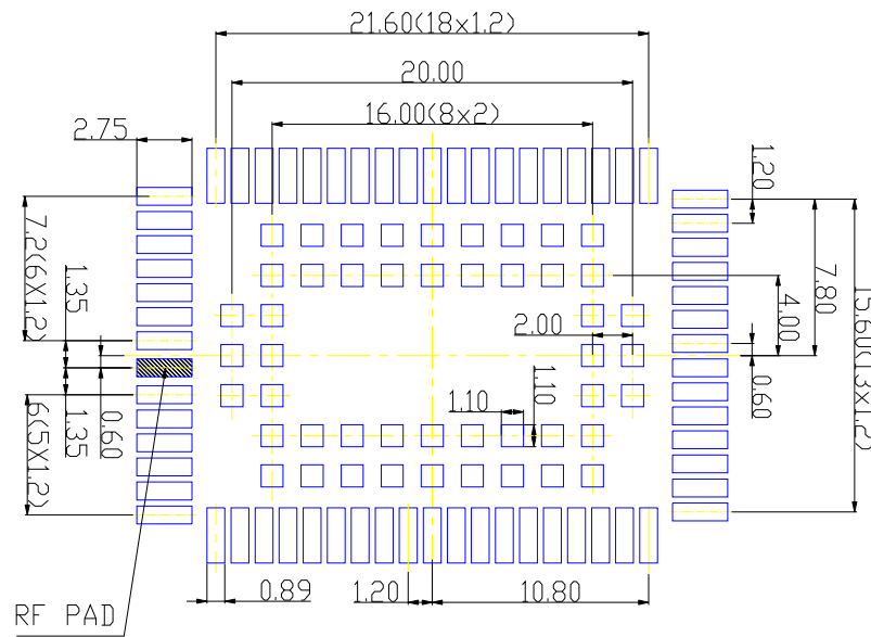
Figure 41: Recommended design for 120 micron thick stencil (top view)
