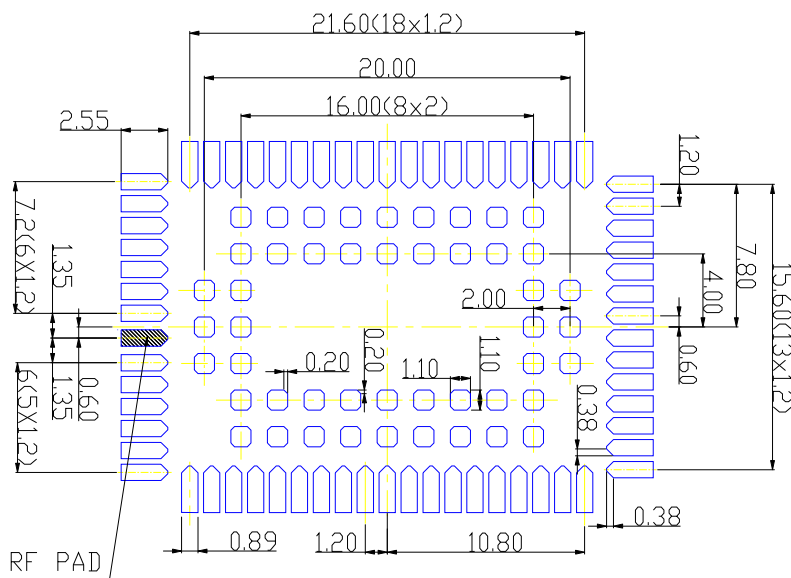
Figure 42: Recommended design for 150 micron thick stencil (top view)
