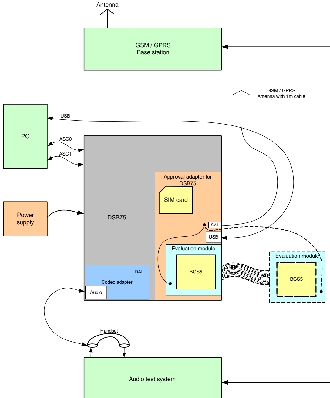
Figure 54: Reference equipment for Type Approval
