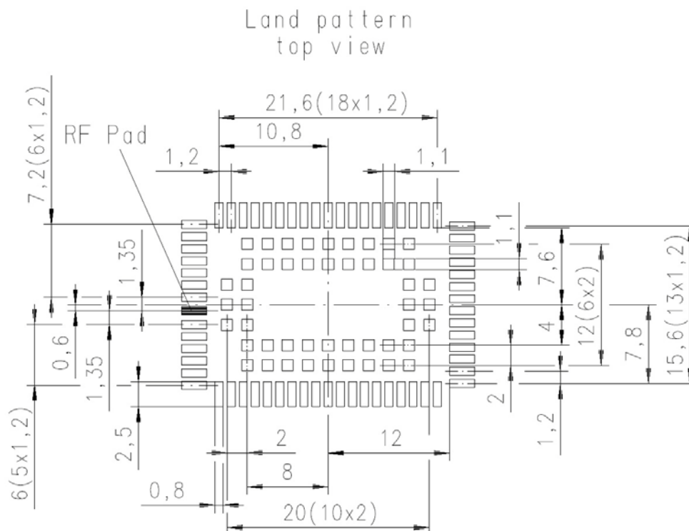
Figure 40: Land pattern (top view)
